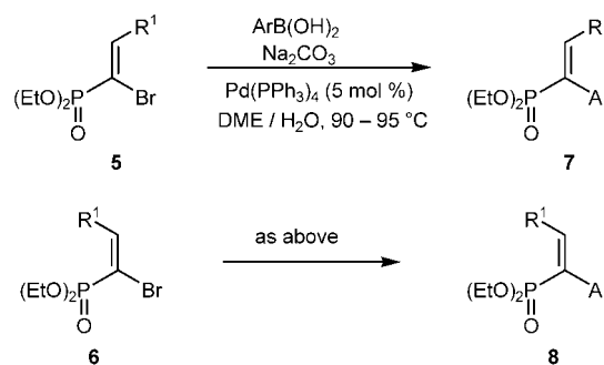
Scheme 3. Arylation of \alpha -bromoalkenylphosphonates. R^1 for 5–8 : a , Me; b , \text{C}_5\text{H}_{11} ; c , Ph.
