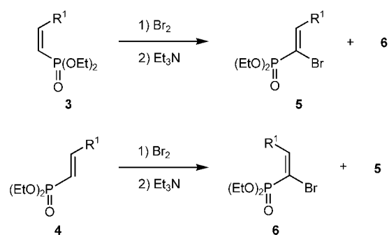
Scheme 2. Preparation of \alpha -bromoalkenylphosphonates. R 1 for 3–6: a , Me; b , C 5 H 11 ; c , Ph.
