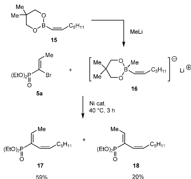
Scheme 5. Alkenylation of a more congested combination.
