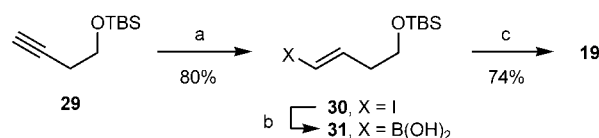
Scheme 7. Synthesis of boronate ester 19 . (a) Cp_2ZrCl_2 , LiBHET_3 then I_2 ; (b) (i) n -BuLi, (ii) B(O-i-Pr)_3 , (iii) H_2O ; (c) Me_2C(CH_2OH)_2 , MgSO_4 .
