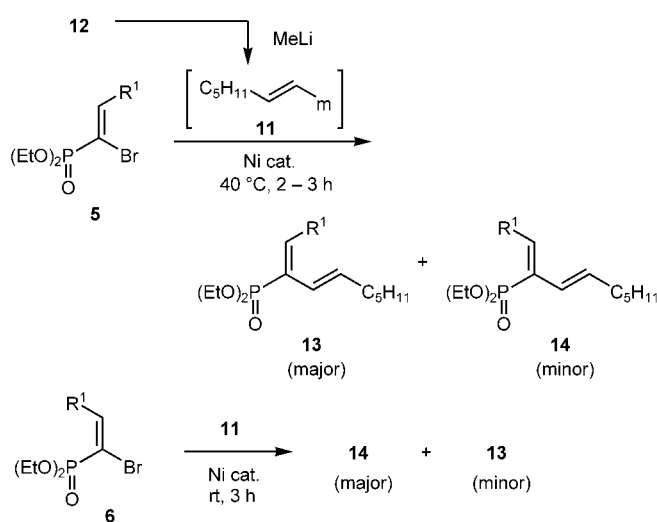
Scheme 4. Alkenylation of bromides 5 and 6 with ( E )-alkenylborate 11 . R^1 for 5 , 6 , 13 , 14 : a , Me; b , C 5 H 11 ; c , Ph.
