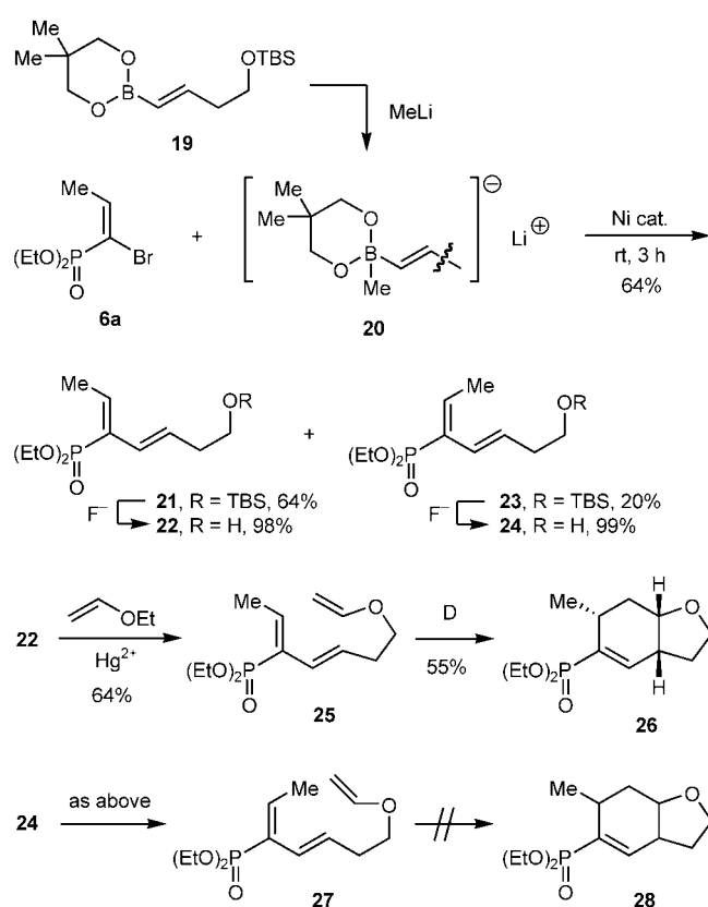
Scheme 6. Synthesis of dienes and their Diels–Alder reaction.
