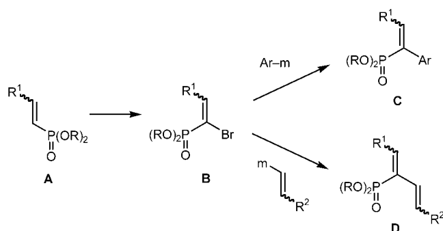
Scheme 1. Carbon-carbon bond formation at the \alpha -position of alkenylphosphonates.
