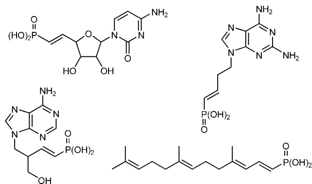
Figure 1. Biologically active alkenylphosphonic acid derivatives.
