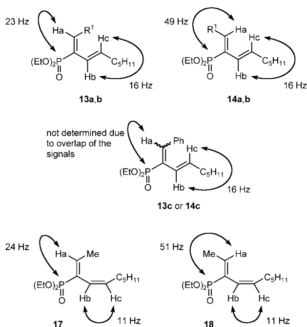
Figure 2. Coupling constants of dienes. R^1 : a , Me; b , C_5H_{11} , c , Ph.
